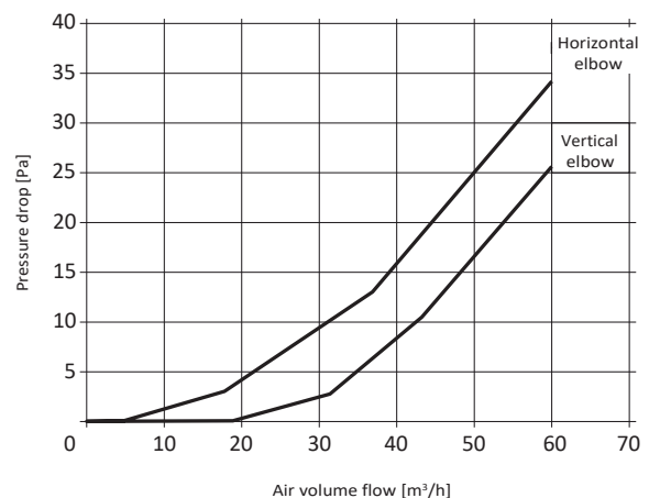
Pressure loss chart for a 90° elbow
